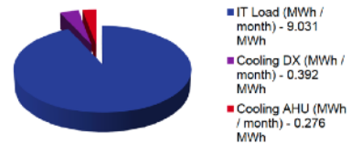
Electricity consumption_July_2017_New system based on DX_AHU (Free Cooling and PCM)
